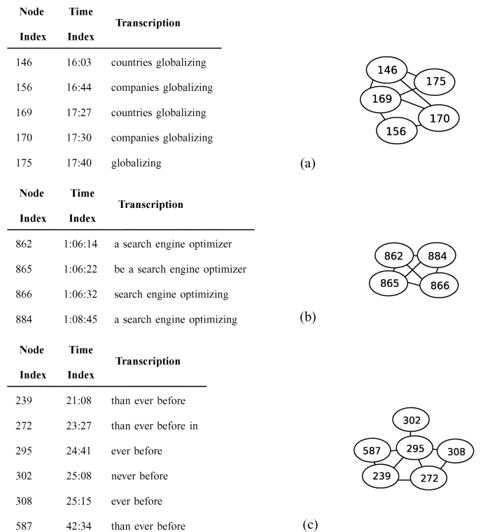
Fig. 9. Detailed view of clusters 17, 24, and 10, including the node indices, transcriptions, and locations in the audio stream.
