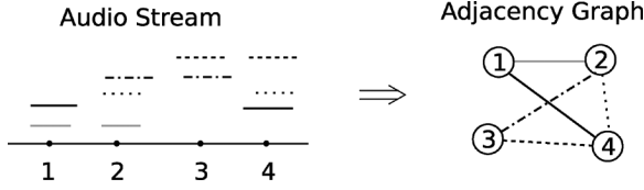
Fig. 6. Production of an adjacency graph from alignment paths and extracted nodes. The audio stream is shown as a timeline, while the alignment paths are shown as pairs of colored lines at the same height above the timeline. Node relations are captured by the graph on the right, with edge weights given by the path similarities.
