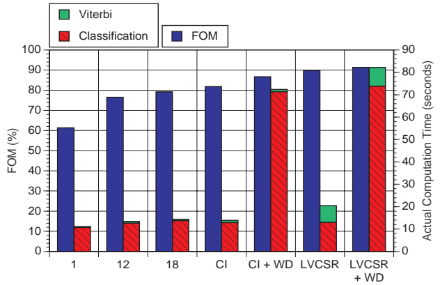
Figure 4: FOM and computation time measurements for all developed word spotters.
