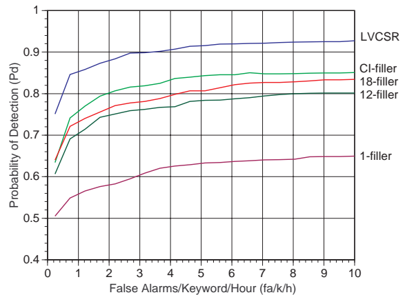
Figure 2: ROC-curves
