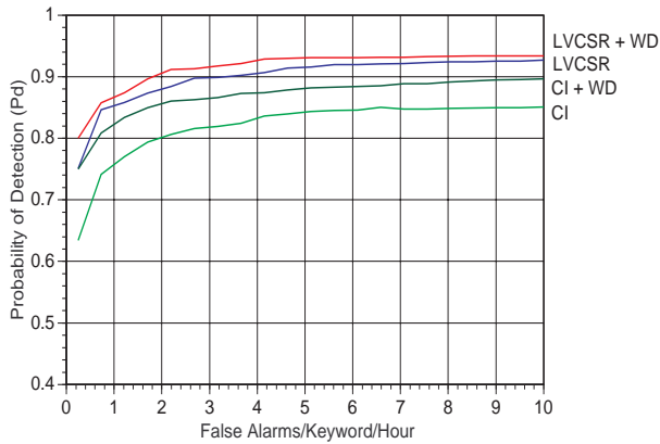
Figure 3: ROC-curves
