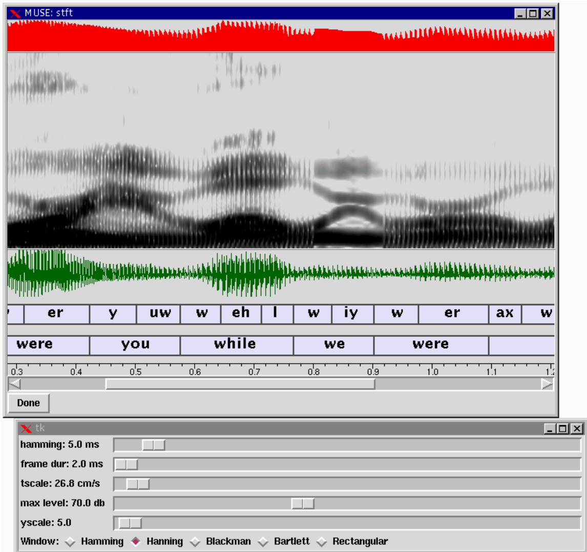
Figure 5-1: A spectrogram editor.
