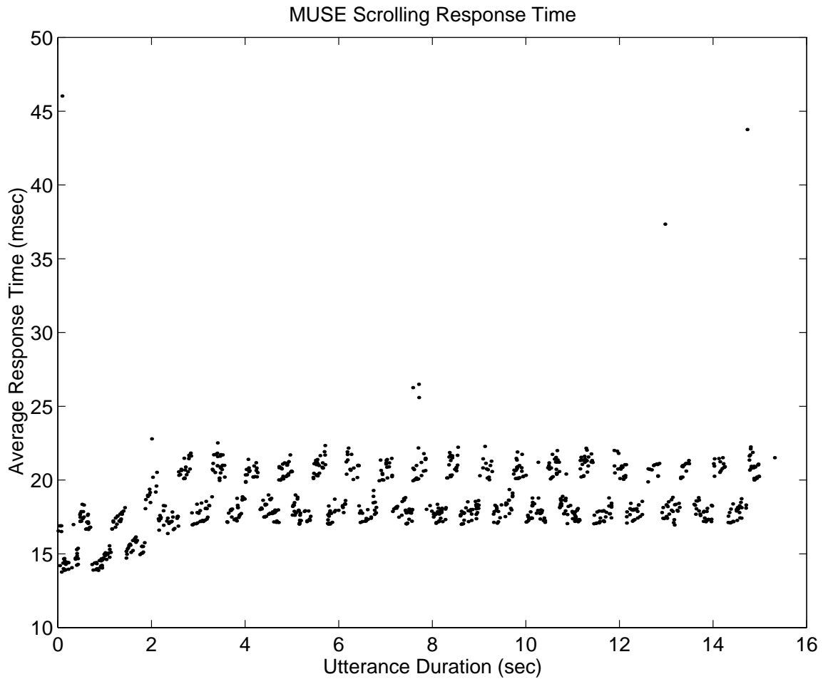
Figure 5-12: Average response time for 1000 scrolling trials for MUSE.
