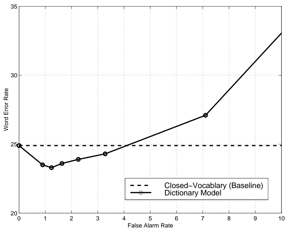
Figure 4-17: WER on the HUB4 test set. Shown is the closed-vocabulary performance (24.9%) and the performance of the dictionary model system as a function of the FAR.
