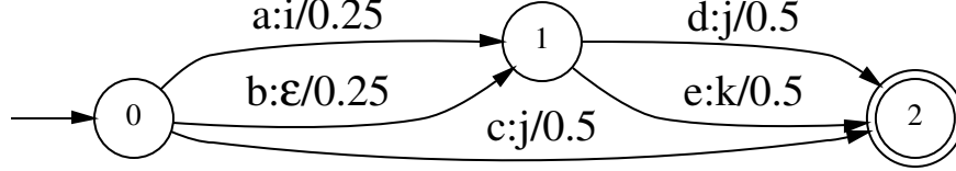
Figure 2-5: An example weighted finite-state transducer. The input alphabet is a, b, c, d, e. The output alphabet is i, j, k. There are three states, labelled 0, 1, 2. The initial state is 0, and the set of final state is 2. The arcs are each labelled with input label : output label / weight . There are a total of five possible paths represented by this FST. The path with the state sequence 0, 2 has the highest weight which maps the input sequence c with the out sequence with the weight of 0.5.
