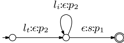
Figure 6-6: Model Topology M^{(q)} for 2-stream landmark/segment phonetic model using mFST. The single stream landmark model is a 2-state HMM, l_t is the transition model, and l_i is the internal model. The single stream segment model is a 1-state whole-segment model s .
