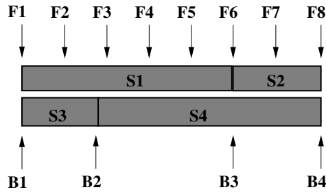
Figure 2-3: Examples of frame-based, landmark, and segment features. The feature vectors, F_1, F_2, \dots, F_8 , are the frame-based which are sampled at fixed-size intervals. The landmark feature vectors, B_1, B_2, B_3 , and B_4 are sampled at variable size intervals. The segment feature vectors, S_1, S_2, S_3 , and S_4 , each spanning two landmark features.
