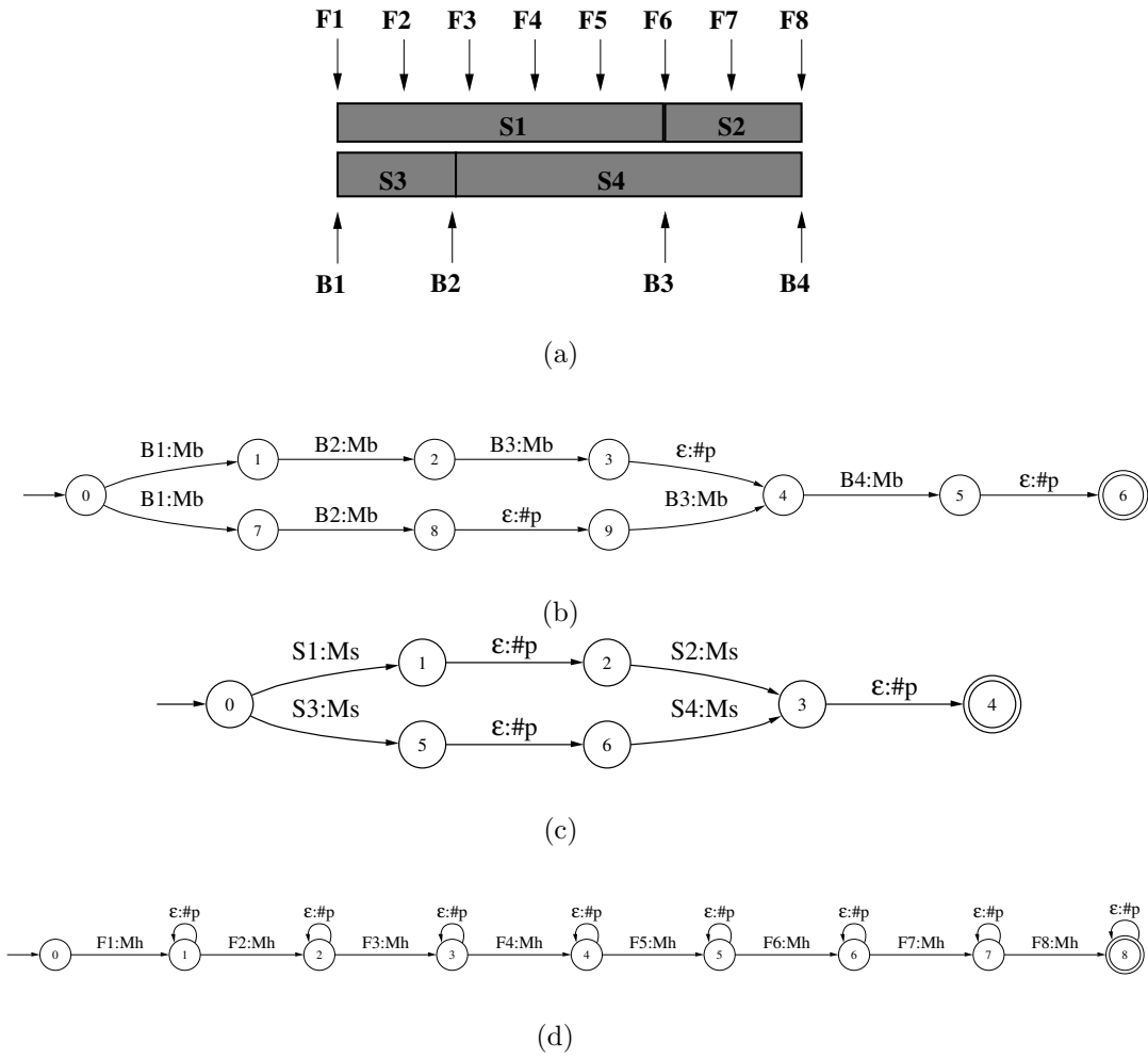
Figure 4-2: Illustration of a sample segmentation network and its corresponding FST representation. Here only the FST A_S is shown since FST A_M simply translates the output symbol Mb , Ms , Mh into the set of all possible sub-phone states. The segmentation network in (a) contains four phonetic segments with four landmark feature vectors, B1 , B2 , B3 , and B4 , and four segment feature vectors, S1 , S2 , S3 , and S4 . The feature vectors, F1 , F2 , \dots , F8 are the corresponding fixed frame-rate feature vectors using by HMMs. (b) shows the corresponding FST A_S for landmark features with two identical input sequences, B1B2B3B4 , and the symbol Mb represents the set of all landmark models. The symbol \#p denotes phone landmark locations. (c) shows the corresponding FST A_S for segment features with two different input sequences each with two segments, S1S2 and S3S4 , and the symbol Ms represents the set of all segment models. (d) shows the corresponding FST A_S for a frame-based HMM. Since the symbol \#p in (d) does not provide any constraint, the size of the corresponding A = A_S \circ A_M is typically bigger than that of segment-based models in (b) and (c). It is important to note the all the input sequences for landmark models as illustrated in (a) are the same, where the input sequences for segment models as illustrated in (b) can be different.
