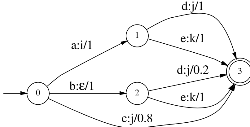
(c) T_{X|Y}
