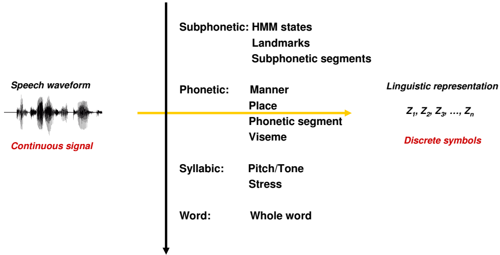
Figure 1-2: Various feature streams for automatic speech recognition.
