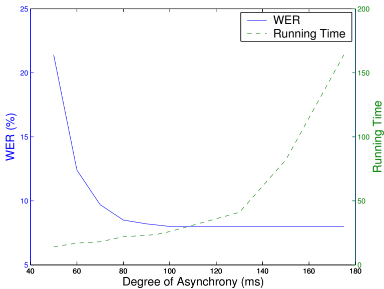
Figure 6-8: WERs and decode time vs. degree of asynchrony.
