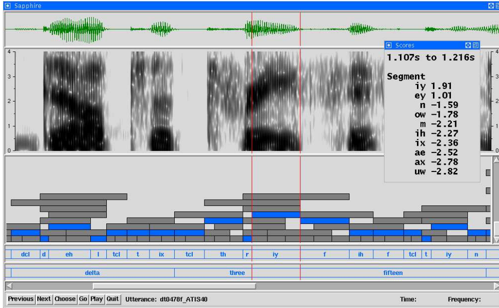
Figure 2-4: Graphical output from the SUMMIT segment-based ASR system. The top two panels display the speech waveform and corresponding spectrogram, respectively. The third panel shows the computed segmentation network consisting of hypothesized phonetic segments. The highlighted segments form a single segmentation path, which is also the segmentation path the decoder found to have the highest score. The fourth panel shows the hypothesized phone sequence aligned to the highlighted segmentation path from the previous panel. The fifth panel shows the corresponding hypothesized word sequence.
