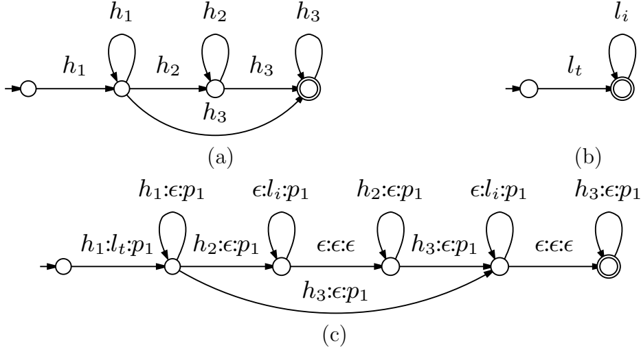
Figure 6-7: (a) Model topology a single-stream HMM. (b) Model topology a single-stream landmark model. (c) Model Topology M^{(q)} for the 2-stream landmark and HMM system using mFST. It is a combination of the single-stream FSTs shown in (a) and (b). Other configurations of the mFST are possible, including a full Cartesian product. (c) shows the topology used in our experiments.
