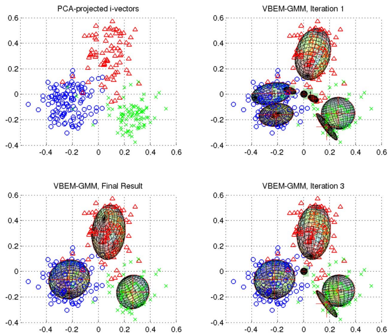
(Top Left) A visualization of the first two principal components of the i-vectors in a three-speaker conversation. The rest of the plots show the result of VBEM-GMM clustering after a single iteration (top right), three iterations (bottom right), and the final results (bottom left). For more see "Unsupervised Methods for Speaker Diarization: An Integrated and Iterative Approach," by Shum et al. , p. 2015.
