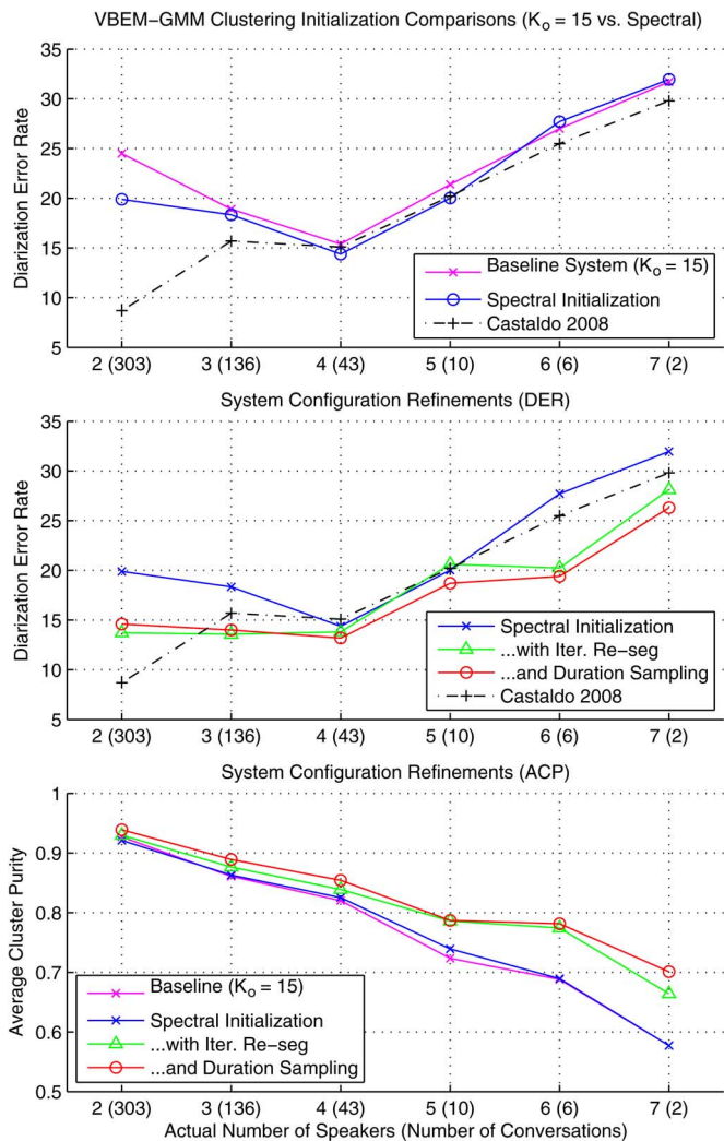
Fig. 3. (Top) results comparing the baseline initialization of VBEM-GMM using K_0 = 15 , in magenta, with an initialization using the spectral clustering heuristic described in Section V-A, in blue. (Middle) results obtained after incorporating the various system refinements proposed in Section V. In blue is our baseline that initializes VBEM-GMM using the spectral clustering heuristic (same as the plot on top). We show the state-of-the-art benchmark results from [14] in black. (Bottom) for each of the systems whose DER results we show above, we also show its Average Cluster Purity (ACP) using the same line color coordination and similar marker type.
