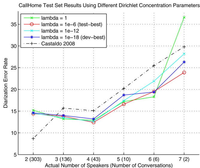
Fig. 6. Results on CallHome test set using different values for the Dirichlet concentration parameter, \lambda_0 .
