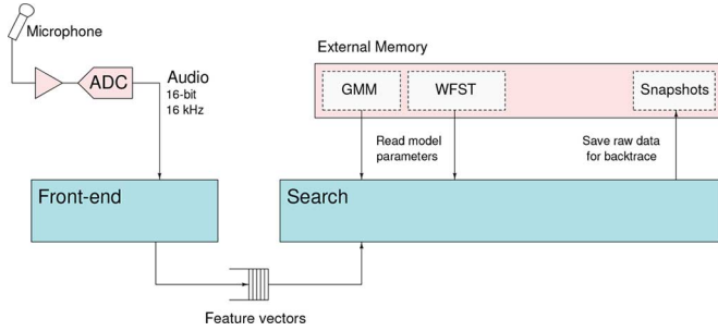
Fig. 2. High-level architecture of speech decoder.
