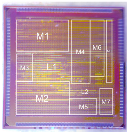
Fig. 10. Annotated die photo of speech decoding chip.
