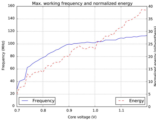
Fig. 13. Voltage/frequency scaling performance.
