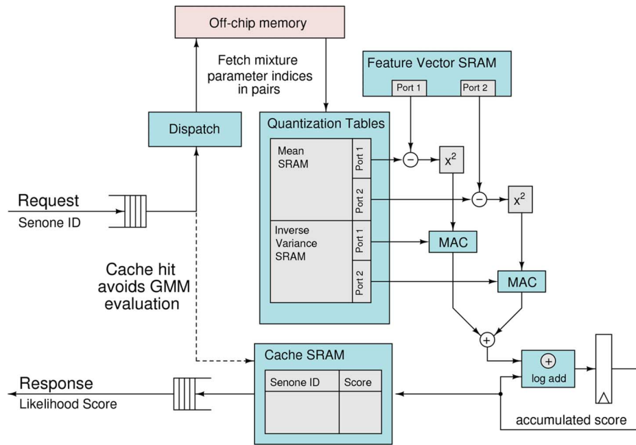
Fig. 9. Block diagram of GMM evaluator incorporating caching and parameter quantization.
