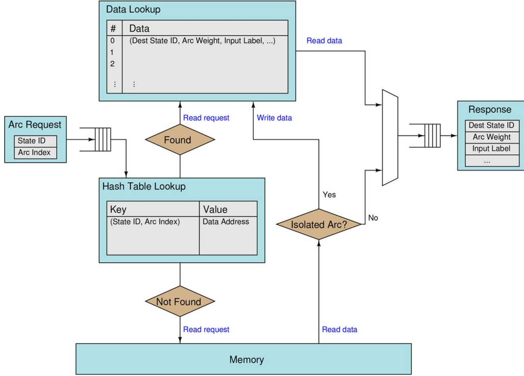
Fig. 7. Block diagram of WFST arc cache.
