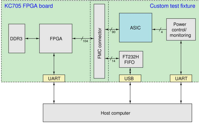
Fig. 12. Block diagram and photograph of test setup.
