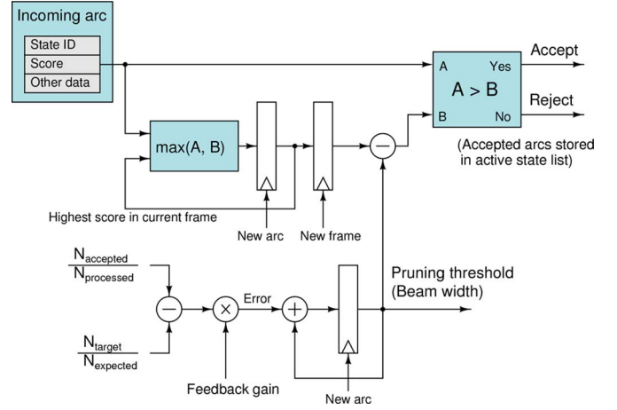
Fig. 5. Block diagram of feedback-based beam width controller.
