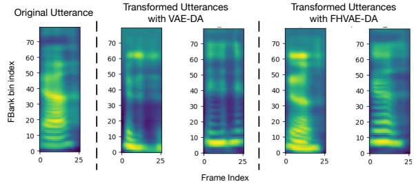
Figure 1: Comparison between VAE-DA and proposed FHVAE-DA applied to a short utterance using nuisance factor replacement. The same source and two target utterances are used for both methods. Our proposed FHVAE-DA can successfully transform only nuisance factors, while VAE-DA cannot.
