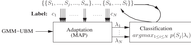
Fig. 3. Illustration of segment-based clustering for speech data with N classes.
