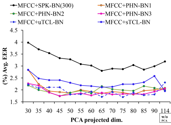
Fig. 8. The TD-SV performance for various dimensions of PCA projected augmented feature (MFCC+BN) of different systems on the m-part-01 task of the RedDots database using GMM-UBM.
